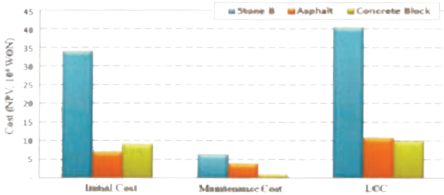
Figure 9) LCCA results of pavement during 40years
